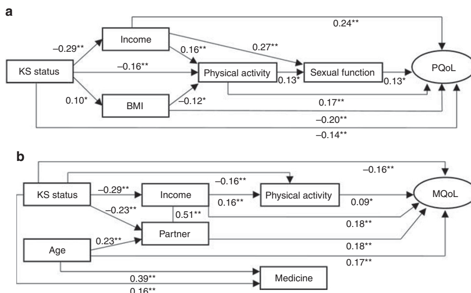
Figure 3 Path models. Physical quality of life (PQoL; a ) and mental quality of life (MQoL; b ) with \beta standard coefficients. PQoL and MQoL are latent variables. The rectangles represent observed variables. BMI, body mass index; KS, Klinefelter syndrome. ^*P < 0.05 , ^{**}P < 0.01 .
